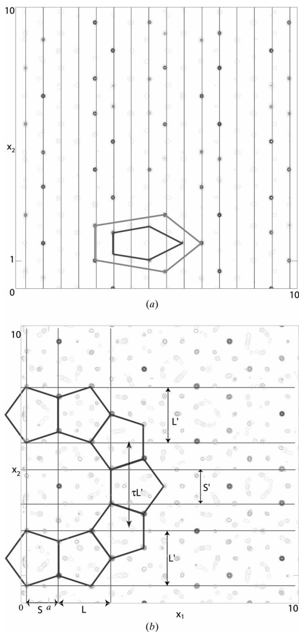
Figure 5 (a) Structure of the net plane (0\bar{1}\bar{1}01) . (b) Quasiperiodic atomic layer of decagonal Al-Co-Ni with x_3 = 1/4 (Cervellino et al. , 2001). Some geometrical structure motifs and unit lengths are marked.
