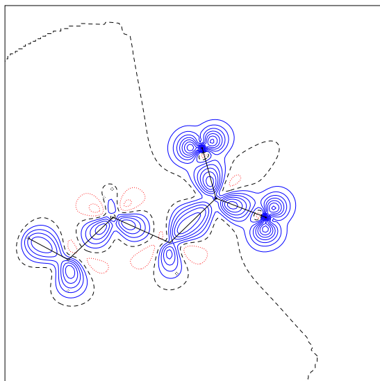
Figure 1: Static deformation density of the predicted charge density in the molecular plane of sarcosine calculated using N1 O1 and O2; contour lines with 0.1 e \cdot \text{\AA}^{-3} steps, blue = positive, red = negative, zero contour dashed.
