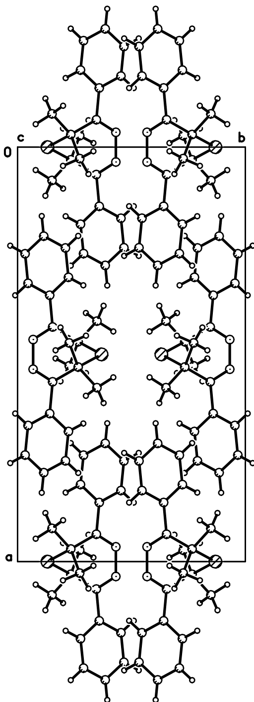
Supplementary Fig. 2. View of the structure looking down the c axis showing the directly analogous packing in the isomorphous crystals [space group Pbcn , Z = 4] of cyclic thioether (I).
