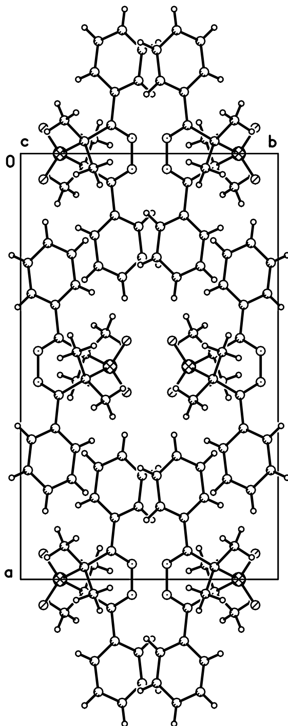
Supplementary Fig. 2. View of the structure looking down the c axis showing the directly analogous packing in the isomorphous crystals [space group Pbcn , Z = 4] of sulfone (II).
