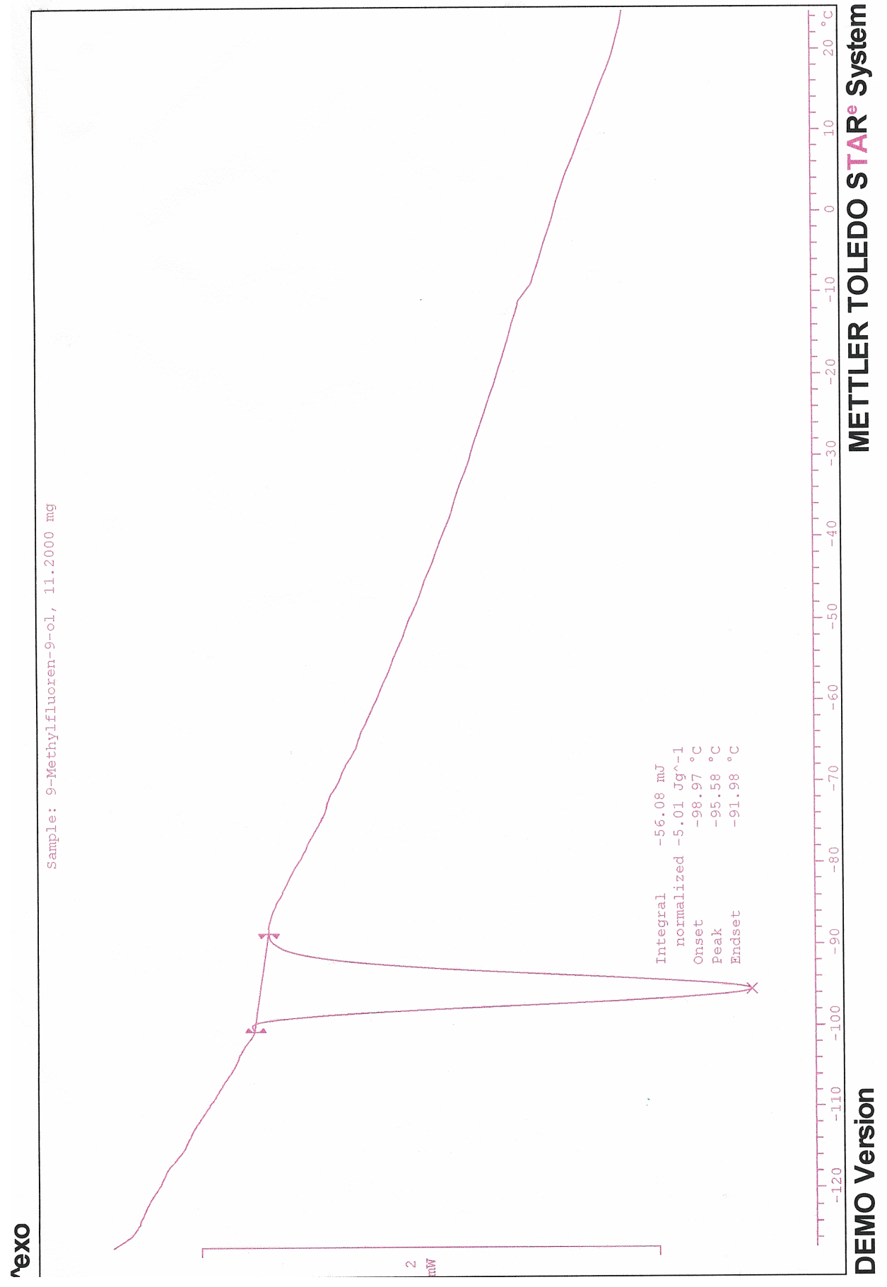
Figure 4 (for deposition). Differential scanning calorimetry trace for 9-methyl-9-fluorenl.
