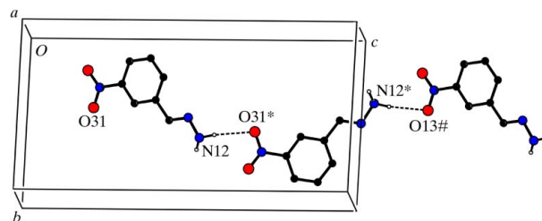
Figure 3 Part of the crystal structure of (II), showing the formation of a C(9) chain along [001] . For the sake of clarity, H atoms bonded to C atoms have been omitted. Atoms marked with an asterisk (*) or a hash (#) are at the symmetry positions (\frac{1}{2} - x, 1 - y, \frac{1}{2} + z) and (x, y, 1 + z) , respectively.
