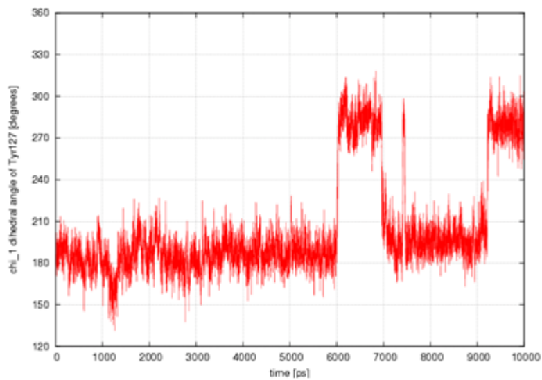
Time evolutions of \chi_1 dihedral angle of Tyr127 in the MD simulations of unliganded (upper panel) and liganded NikA (lower panel).
