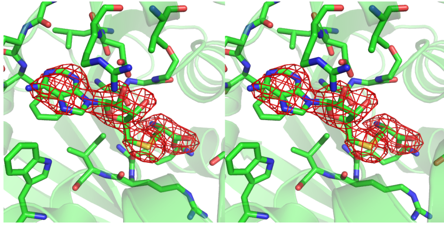
Supplementary Figure 1. Simulated annealing OMIT F_o - F_c electron-density map for the SAH-binding region. The contour level is at 3\sigma .
