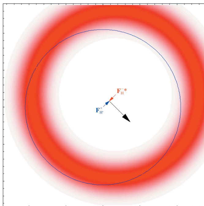
Figure 3 The probabilistic Harker construction for SAD phasing. For this figure, the base of the \mathbf{F}_H^{+''} vector is chosen as the origin. Uncertainty in the anomalous scatterer model will lead to uncertainty in the scale and orientation of the set of black, red and blue vectors representing the real and imaginary contributions of the anomalous scatterers to \mathbf{F}^+ and \mathbf{F}^{-*} . This leads to uncertainty in the position of the red circle, which is represented as a circular distribution of red shading. The contribution of errors in the measurement of the observed |F_o^+| and |F_o^-| can be represented as a further increase in the width of the red distribution.
