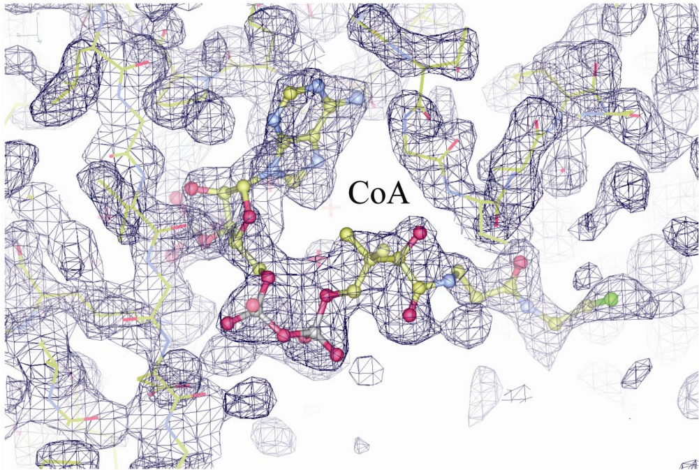
Supplementary Figure 1. Experimental density map (AcpS VC structure) after density modification countered at 1.28 \sigma .
