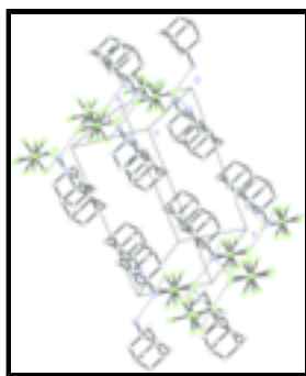
Fig. 2. Unit-cell contents.
