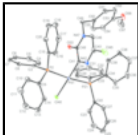
Fig. 1. The molecular structure of the title compound (I), showing the atom-labeling scheme with displacement ellipsoids drawn at the 50% probability level. H atoms have been omitted for clarity.
