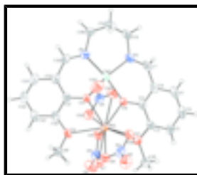
Fig. 1. The molecular structure, showing 40% probability displacement ellipsoids for non-H atoms. The acetone solvent molecule is not shown.
