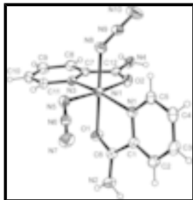
Fig. 1. The ORTEP-3 drawing of (I) with the atom numbering scheme. Displacement ellipsoids for non-H atoms are drawn at the 30% probability level.
