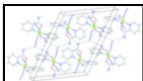
Fig. 2. Crystal packing of (I) showing the hydrogen bonds as dashed lines.
