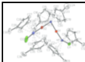
Fig. 1. The molecular structure of ( 1 ), with atom labels and 50% probability displacement ellipsoids for non-H atoms.
