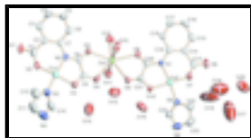
Fig. 1. Asymmetric unit of the title compound. Hydrogen atoms are omitted for clarity. Displacement ellipsoids are drawn at the 50% probability level.
