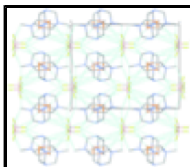
Fig. 2. Partial representation (view along the b axis) of the crystal packing diagram of (I) showing the generation of the three-dimensional supramolecular assembly via C-H\cdots F hydrogen bonds and C\cdots F short contacts (blue dotted lines). Hydrogen atoms and disordered F1B and F3B atoms are omitted for clarity. C, grey; N, blue; P, orange; F, light green; B, pink.
