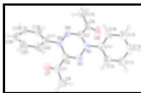
Fig. 1. The molecular structure of (I) showing 50% displacement ellipsoids (arbitrary spheres for the H atoms).
