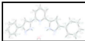
Fig. 1. The molecular structure of the title compound, showing the atom-numbering scheme. Displacement ellipsoids are drawn at the 40% probability level. H atoms are shown as small spheres of arbitrary radii.
