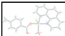
Fig. 1. The structure of (I), showing the atomic numbering scheme. Non-H atoms are shown with 30% probability displacement ellipsoids.
