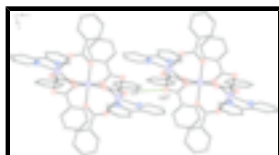
Fig. 2. The intermolecular C-H \cdots O hydrogen bond between the molecule units. H atoms not included in the hydrogen bond were omitted for clarify. Symmetry codes: (ii) 2-x, 2-y, 1-z .
