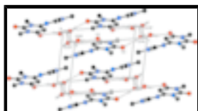
Fig. 2. A packing diagram for (I), viewed down the b axis. H atoms not involved in hydrogen bonding have been omitted for clarity. [Symmetry code:(i) -x, -y + 1, -z + 2 ; (ii) x, y, z - 1 ].
