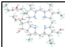
Fig. 1. The molecular structure of the title compound showing the atomic numbering and 70% probability displacement ellipsoids.
