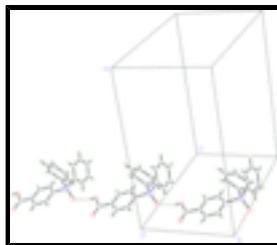
Fig. 2. View of the chain structure of the title compound; hydrogen-bonds are drawn as dashed lines.
