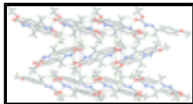
Fig. 2. The crystal packing of the title compound, viewed approximately down the c axis. Hydrogen bonds are shown as dashed lines.
