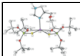
Fig. 1. A view of the title molecule, showing the atom-labelling scheme. Displacement ellipsoids are drawn at the 50% probability level and H atoms, except those from OH and NH groups, have been omitted. Hydrogen bonds are indicated with dashed lines. Only the major conformation for the disordered methyl groups (C24-C25) is shown.
