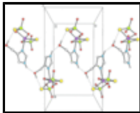
Fig. 2. A view of one-dimensional chains of molecules linked by hydrogen bonds along the c axis. All t Bu groups have been omitted for clarity. Hydrogen bonds are indicated with dashed lines.
