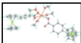
Fig. 1. The molecular structure of (I) at the 50% probability level (arbitrary spheres for the H atoms). The unlabelled atoms are generated by the symmetry operation (1–x, 1+y, 1/2–z).
