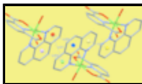
Fig. 2. \pi - \pi interactions between aromatic rings of 1,10-phenanthroline (phen).
