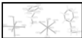
Fig. 1. Molecular structure of (1). Thermal ellipsoids are drawn at 50% probability level.
