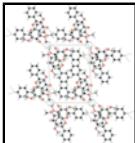
Fig. 2. Part of the crystal structure viewed along the a -axis. Dashed lines represent weak C–H...O interactions.
