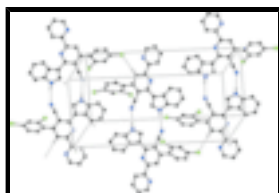
Fig. 2. The crystal packing of the molecules viewed down c axis. H atoms not involved in hydrogen bonding have been omitted for clarity.
