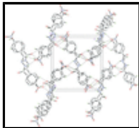
Fig. 2. The packing diagram of the title compound, viewed along the a axis. Hydrogen bonds are shown as dashed lines.
