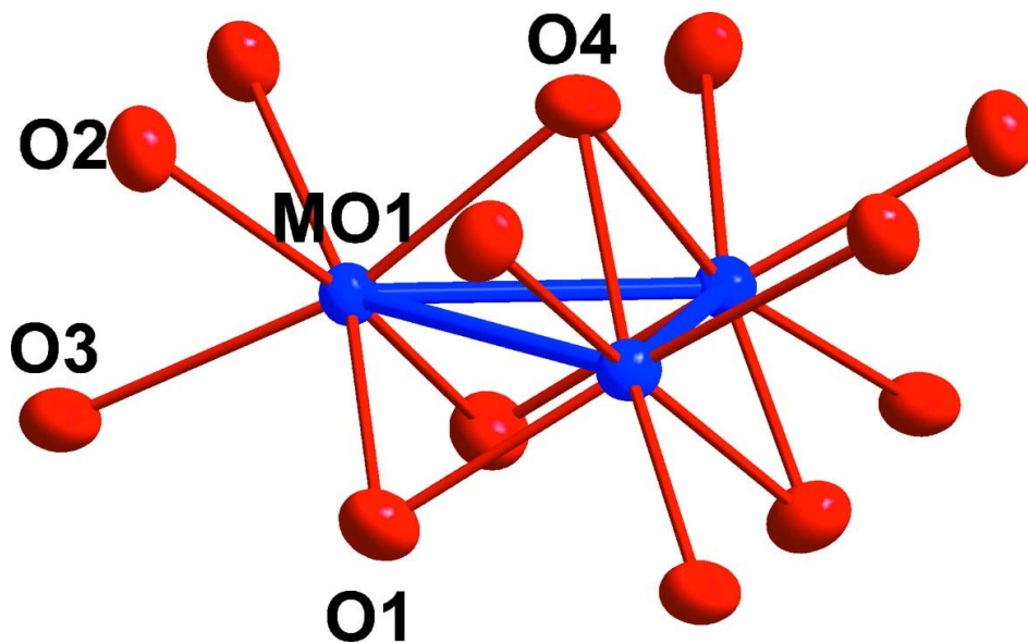
Figure 2 Plot showing the atom-numbering scheme of the \text{Mo}_3\text{O}_{13} cluster unit. Displacement ellipsoids are drawn at the 97% probability level.
