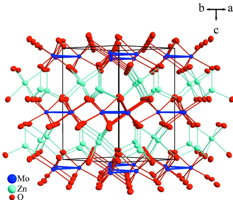
Figure 1 View of \text{Zn}_2\text{Mo}_3\text{O}_8 along [110] .
