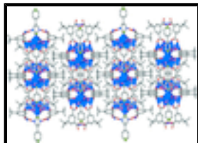
Fig. 3. A perspective view of 1 along c axis. Hydrogen atoms have been omitted for clarity.
