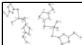
Fig. 1. The molecular structure of (I), showing 30% probability displacement ellipsoids and atom labelling.
