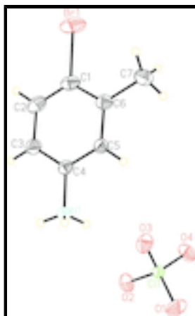
Fig. 1. The molecular structure of the title compound, with the atomic numbering scheme. Displacement ellipsoids are drawn at the 30% probability level.
