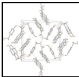
Fig. 2. The packing of (I), showing intermolecular hydrogen bonds (dashed lines) along the a axis.
