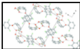
Fig. 2. The crystal packing of (I) viewed along the a axis. H atoms not involved in hydrogen bonds (dashed lines) were omitted for clarity.
