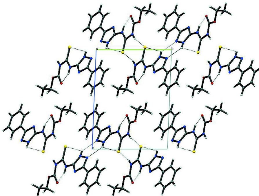
Figure 4 Crystal packing in the cell (view along axis a ).
