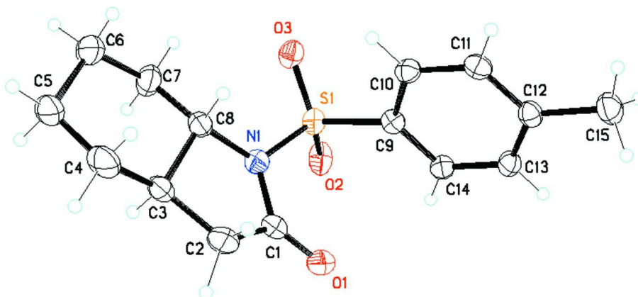
Figure 1 Structure of (I) with 30% displacement ellipsoids.
