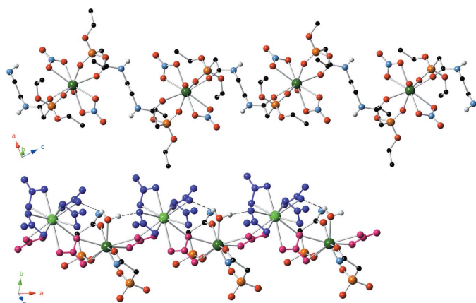
Figure 2 (Top) The Sm2 cations of each metal chain are linked to a neighboring metal chain via the di-CMPO organic ligands. Color codes: black C, light green Sm1, dark green Sm2, red O, blue N, and dark orange P. (Bottom) The metal chain showing alternating Sm1 and Sm2 cations, linked through bridging bis-bidentate nitrate groups shown in pink. Non-bridging nitrate groups are shown in purple. Hydrogen bonds between the water molecule on Sm2 and nitrate groups on Sm1 are shown as dashed lines.
