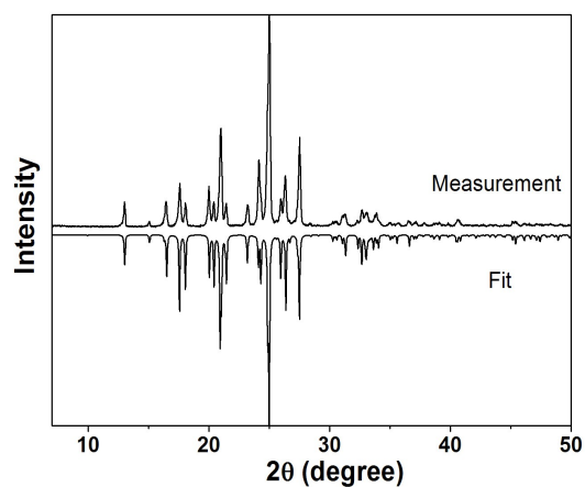
Figure S2. XRD pattern of the powdered sample of 1 . The lower pattern is simulated from the single crystal structure.
