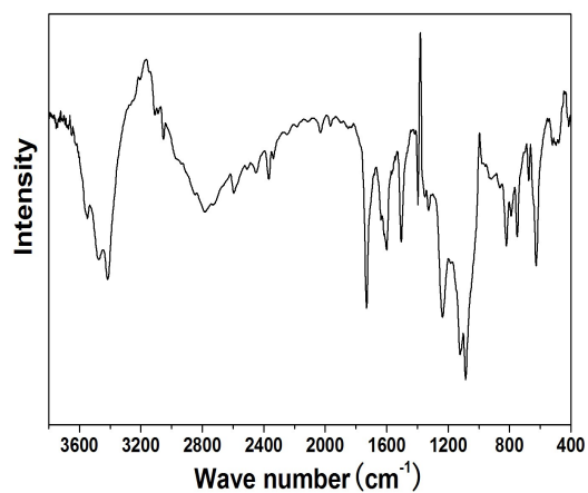
Figure S1 The IR spectrum of 1 .
