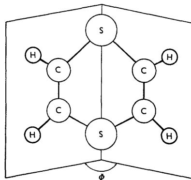
Fig. 8. The molecular structure of 1,4-dithiadene.
