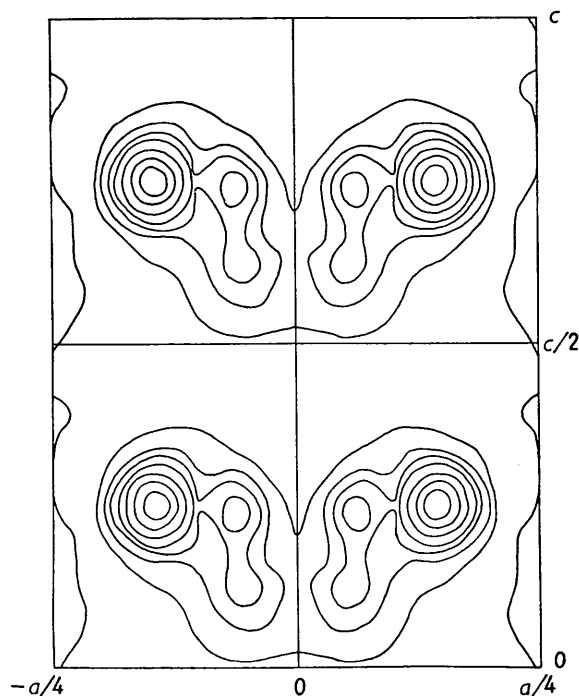
Fig. 3. Projection of electron density along the b axis. Contours are at 0, 2, 4, 6, 8, 12, 16 and 20 e.Å -2 .
