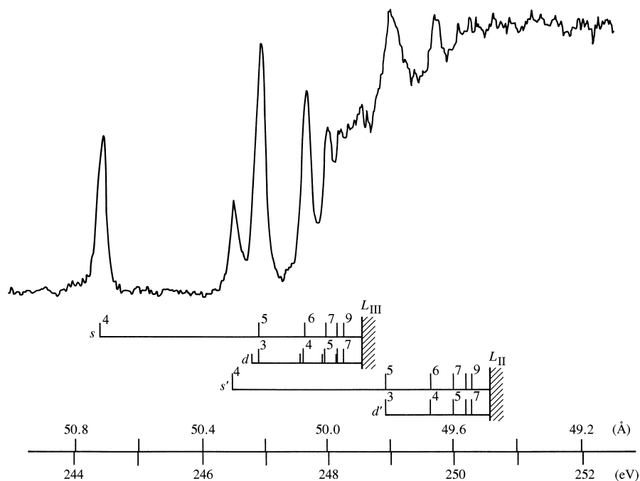
Figure 1 Rydberg series of the argon L_{2,3} absorption spectrum (Nakamura et al. , 1968).
