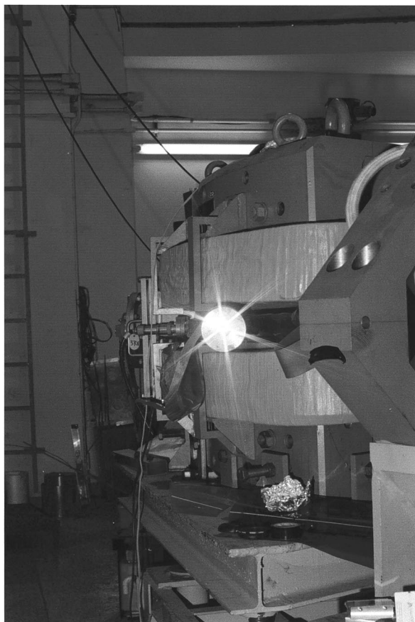
Figure 2 First light from SOR-RING, December 1974.
