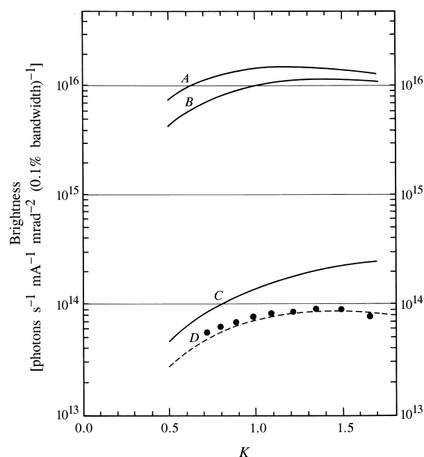
Figure 6 Calculated (A, B, C) and observed (D) peak brightness of 6 cm \times 60 period undulator at BL-2, Photon Factory, against the field parameter K . Curve A is plotted by assuming a low-emittance limit ( <10 nm rad ^{-1} ), B is corrected for a finite aperture, and C is the value for the actual emittance of PF-ring, 400 nm rad ^{-1} . The absolute brightness (D) was deduced from the photoelectron count of helium as the target gas (Sasaki, 1986).
