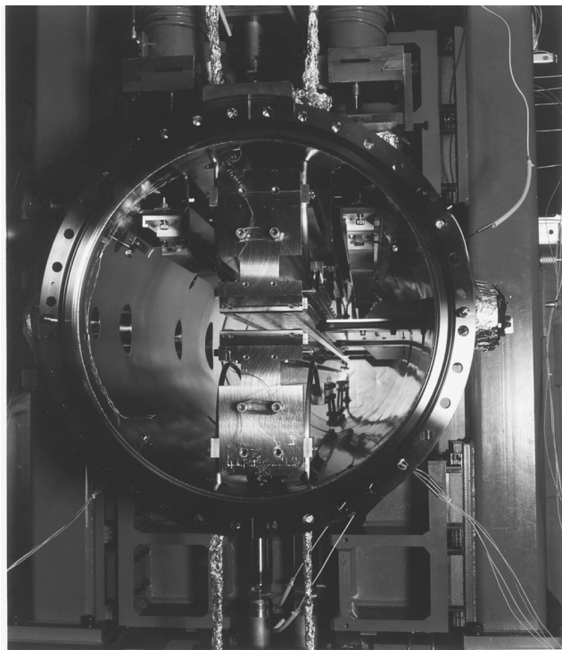
Figure 5 In-vacuum undulator of the 6 GeV TRISTAN AR-ring at the Photon Factory (Yamamoto et al. , 1992).
