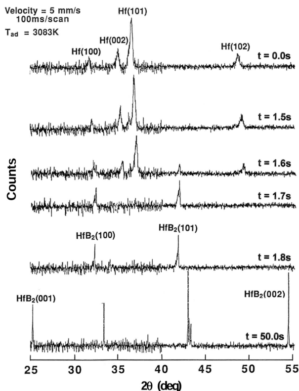
Figure 11 TRXRD patterns for the Hf + 2B \rightarrow HfB_2 reaction, showing the sequence of critical events during the combustion. Hf metal melted and the combustion was completed in 0.2 s.
