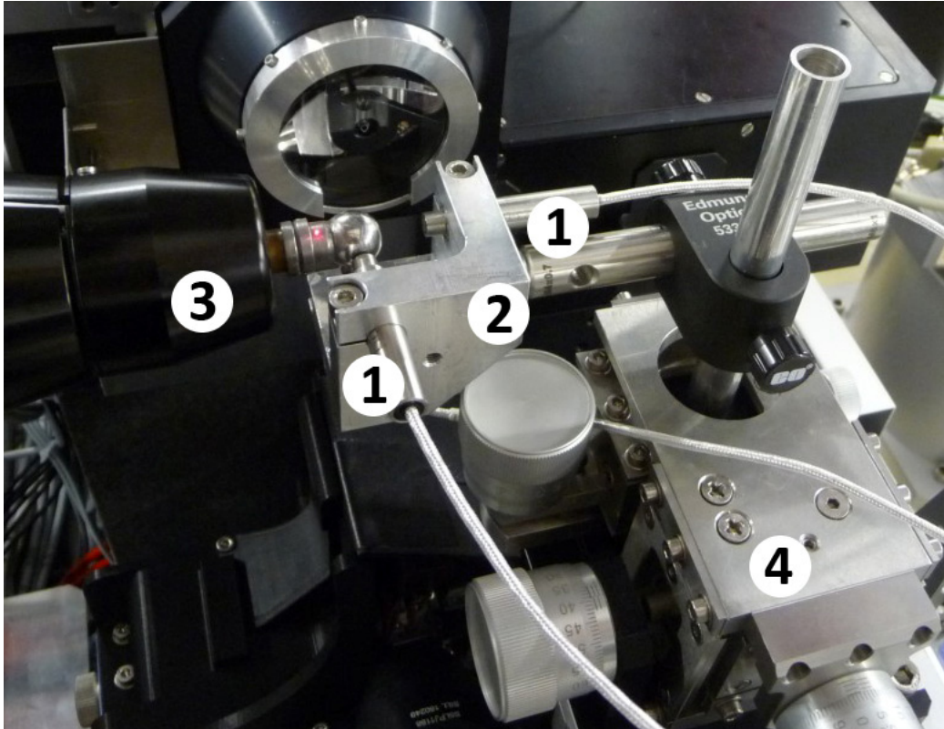
Figure 1 Goniometer metrology setup for cylinder of confusion commissioning. Three capacitive sensors (1) are mounted in an easy-to-adjust bracket (2), one for each spatial direction. The sensors measure the distance to the reference sphere at the sample position. The sphere is centered by the goniometer's centering stages (3) and the capacitive sensors are manually adjusted by an XYZ stage (4).
