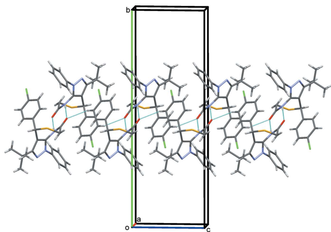
Figure 2 A partial view along the a axis of the crystal packing of the title compound, with hydrogen bonds shown as dashed lines (see Table 1).
