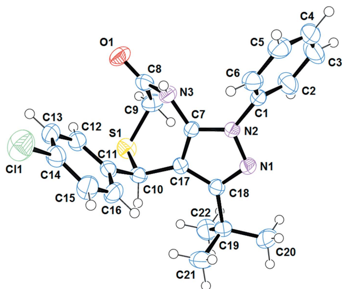
Figure 1 The molecular structure of the title compound, with atom labelling and displacement ellipsoids drawn at the 50% probability level.
