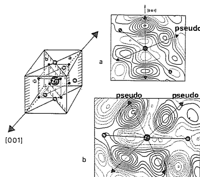
Section of the difference electron density around Zn
