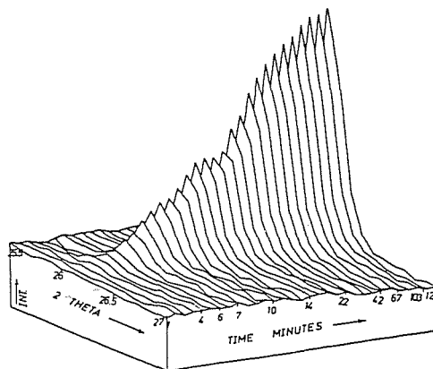
Time resolved XRD study of the nucleation and growth of h-quartz s.s. from \text{Li}_2\text{O}-\text{Al}_2\text{O}_3-\text{SiO}_2 glass at 800^\circ\text{C} .
