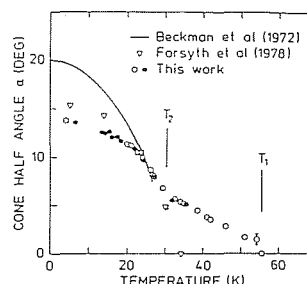
Fig. 1. Cone half angle \alpha in \text{FeGe} (B35) calculated from experimental data assuming a double cone antiferromagnetic structure. The angle \alpha is the angle with which the iron moments are canted away from the c-axis. Also shown are the cone half angles determined by Forsyth et al. and that calculated by Beckman et al.
