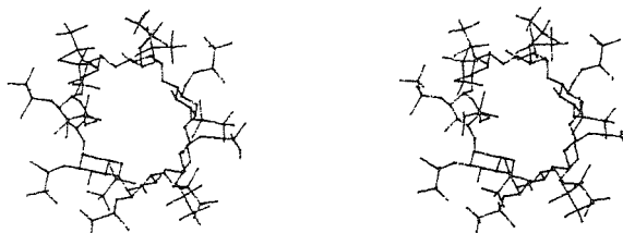
A stereoscopic projection of per-2,6-O- t -butyl-dimethyl-silyl-β-cyclodextrin.
